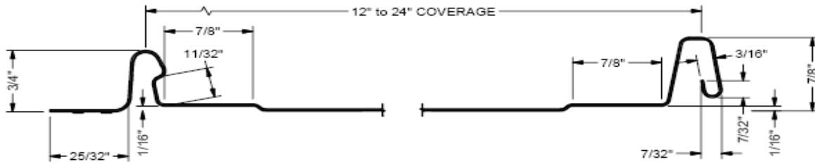
DETAIL A
