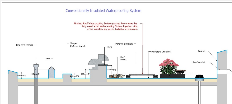
Figure 1.3.2-1 (Conventionally Insulated Waterproofing System)
