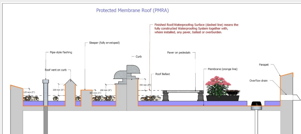
Figure 1.3.2-2 (Protected Membrane Roof Assembly)
