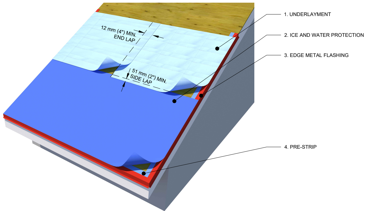
ASM 1.1.1 EAVE PROTECTION and UNDERLAYMENT
