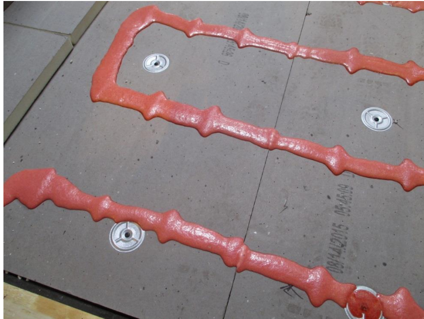
Photo No. 5 12" Bands of Parafast/Olybond
