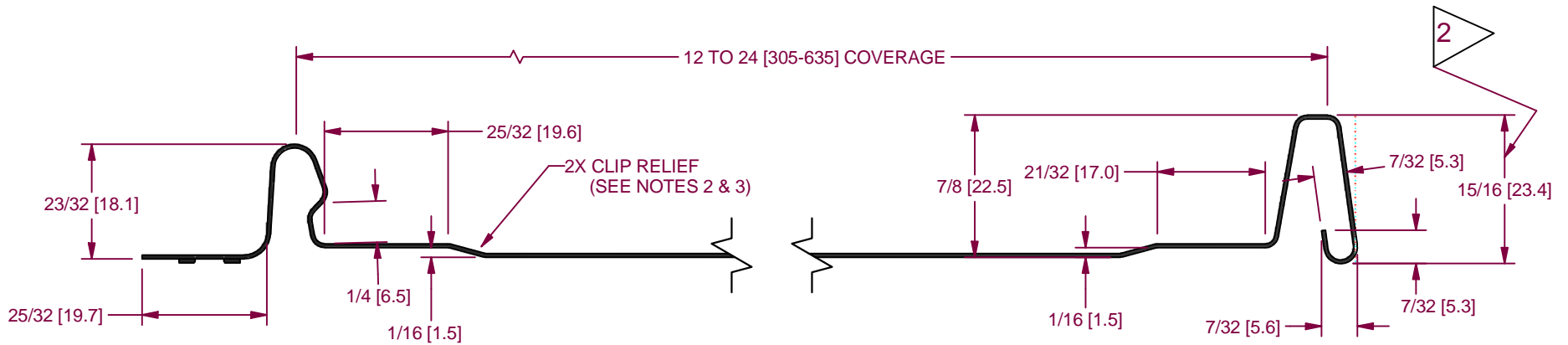
DETAIL A
