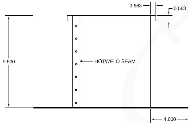
BASE SIDE VIEW
